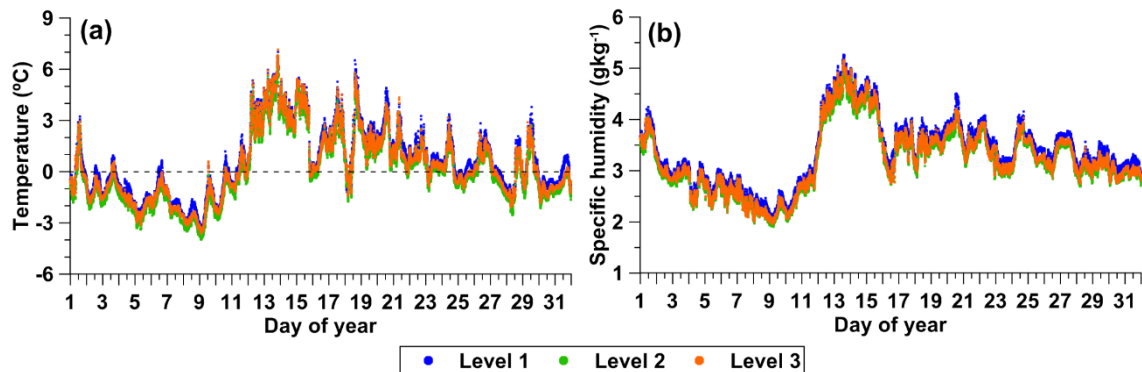
Figure 5: Temporal variation of (a) air temperature (C). The horizontal dashed line indicates 0 C and (b) air specific humidity ( \text{gkg}^{-1} ) for January 2014. Blue, green and orange points represent the values obtained at level 1, 2 and 3, respectively. The data sampling was 10 Hz and it was stored as 5-min average.
